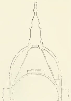
Section of the Dome of St. Paul's.
